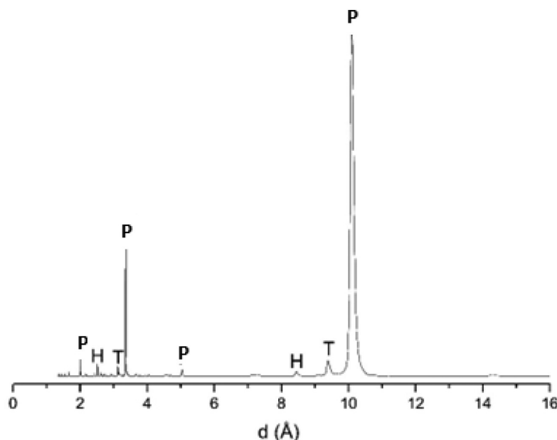
Figure 1. X-ray diffractogram ( \text{Cu}(\text{K}\alpha) ) of the in natura sample. P = Phlogopite ( \text{KMg}_3(\text{AlSi}_3\text{O}_{10})(\text{OH})_2 ), T= magnesium talc ( \text{Mg}_3\text{Si}_4\text{O}_{10}(\text{OH})_2 ) and H= hornblende ( \text{Ca}_2(\text{Mg}_4\text{Fe})\text{Si}_7\text{AlO}_{22}(\text{OH})_2 )
