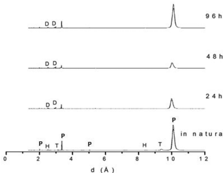
Figure 6. X-ray diffractograms obtained for the in natura sample (Cu(K \alpha )) and submitted to mechanochemical activation (MA) with 10% of CaO for 90 min, calcined at 1,000 °C for 4 h and extracted with C 6 H 8 O 7 at 0.1 mol.L -1 for 24 (Co(K \alpha )), 48 and 96 h (Cu(K \alpha )). P = Phlogopite (KMg 3 (AlSi 3 O 10 )(OH) 2 ), D = Diopside (CaMgSi 2 O 6 ), T = Magnesium talc (Mg 3 Si 4 O 10 (OH) 2 ) and H = Hornblende (Ca 2 (Mg 4 Fe)Si 7 AlO 22 (OH) 2 )
