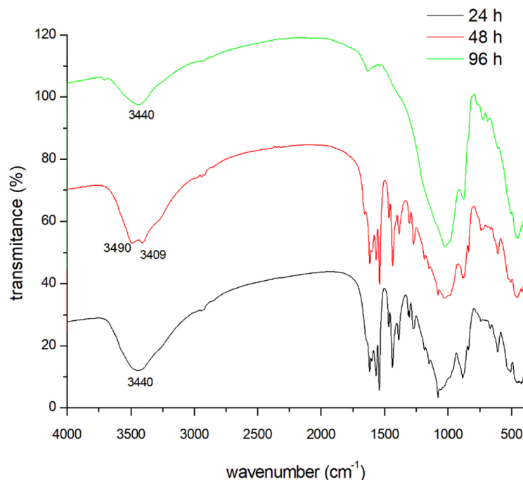
Figure 5. Infrared (IR) spectra obtained for the samples of phlogoptite calcined at 1,200 °C for 4 h with 10% w/w of CaO and submitted to extraction with C_6H_8O_7 at 0.1 mol.L -1 for 24, 48 and 96 h. Reduction of the band at 3,440 cm -1 characteristic of phlogoptite
