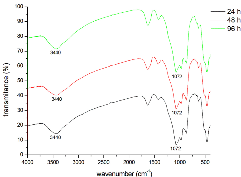
Figure 7. Infrared (IR) spectra obtained from the in natura sample submitted to mechanochemical activation with 10% of CaO for 90 min, calcined at 1,000°C for 4 h followed by extraction with C 6 H 8 O 7 at 0.1 mol.L -1 for 24, 48 and 96 h. Reduction of the band at 3,440 cm -1 , characteristic of phlogopite, and emergence of bands in the 1,100 cm -1 region referring to the glass network rich in silica and modified by CaO
