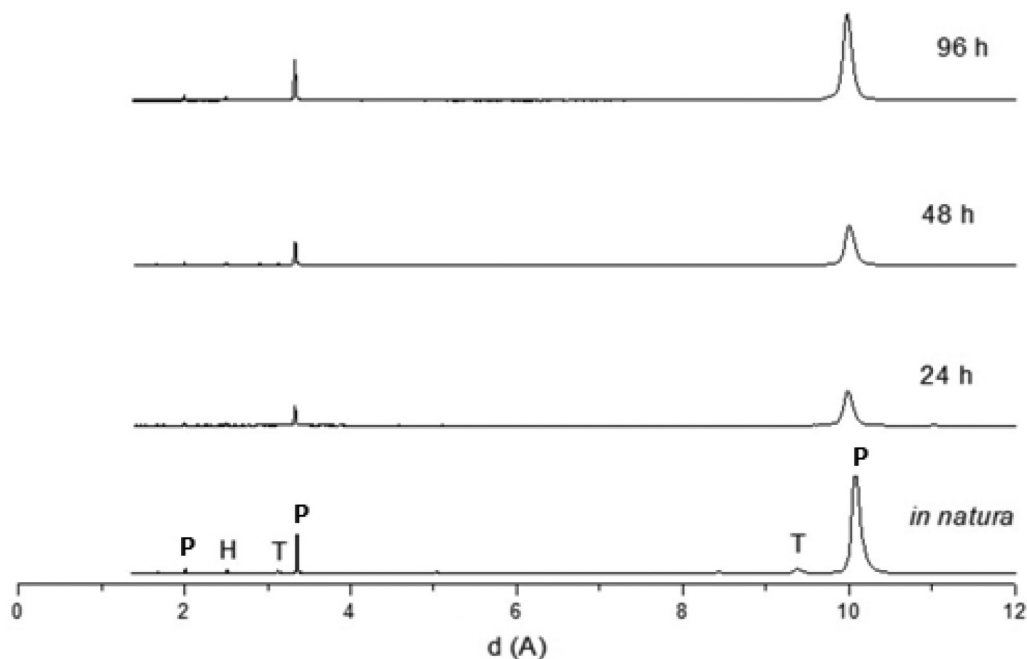
Figure 4. X-ray diffractograms obtained from phlogopite in natura (Cu(K \alpha )) and calcined at 1,200 °C for 4 h with 10% w/w CaO and submitted to extraction with C 6 H 8 O 7 at 0.1 mol.L -1 for 24, 48 and 96 h (Co(K \alpha )). P = Phlogopite (KMg 3 (AlSi 3 O 10 )(OH) 2 ) T= Magnesium talc (Mg 3 Si 4 O 10 (OH) 2 ) and H= Hornblende
