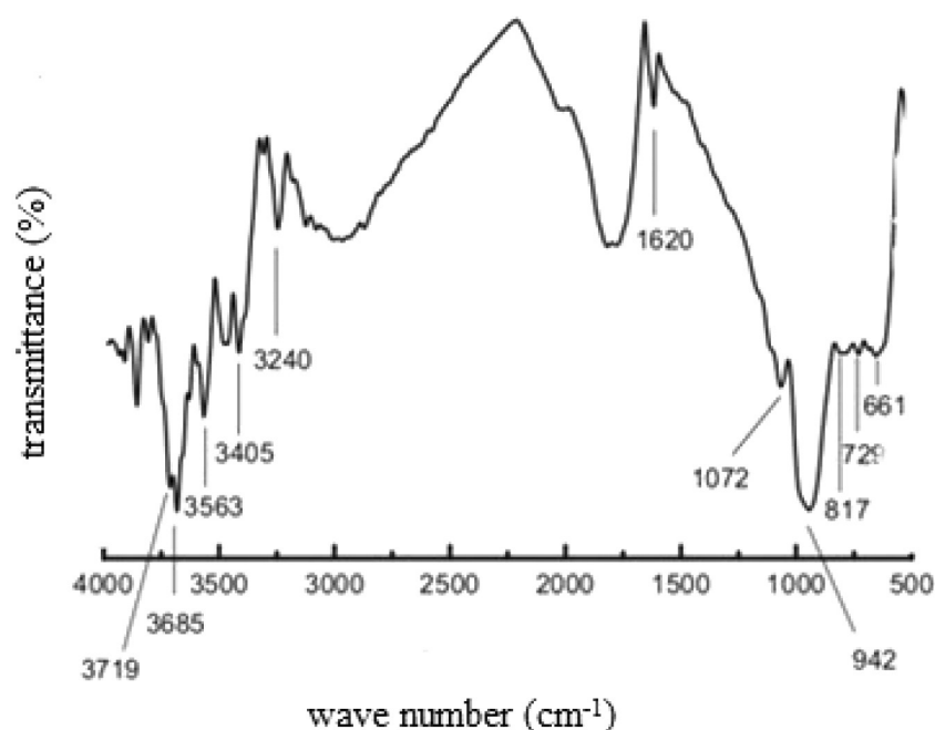
Figure 2. Infrared spectrum of the in natura sample Reprinted from Publication Journal of the Brazilian Chemical Society 2013, 24(8), 1366-1372, Silva, A. A. S.; Sampaio, J. A.; Luz, A. B.; França, S. C. A.; Ronconi, C. M.; Modeling controlled potassium release from phlogopite in solution: exploring the viability of using crushed phlogopite rock as an alternative potassium source in Brazilian soil; doi:10.5935/0103-5053.20130173, with permission from JBCS, PubliSBQ Editorial Manager
