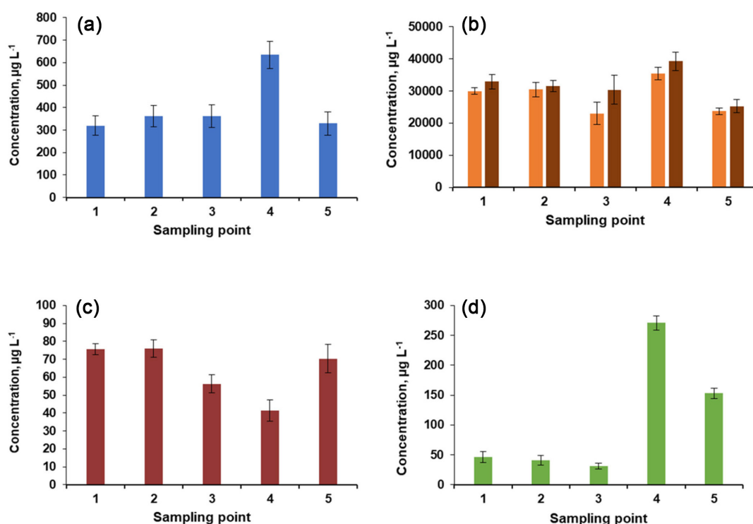
Figure 3. (a) Fluoride, (b) chlorine (orange) and chloride (brown), (c) total bromine, and (d) iodine concentrations determined at each of the 5 sampling points.
