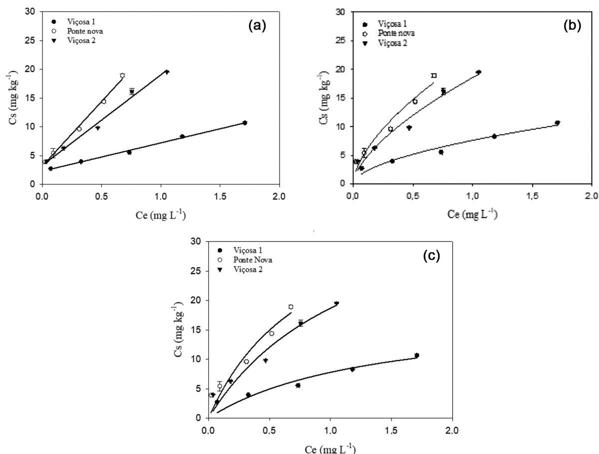
Figure 5. Application of the linear (A), Freundlich (B), and Langmuir (C) desorption isotherm models to the behavior of cyantraniliprole in the different soils
