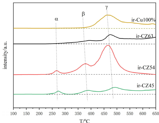
Figure 11. H 2 -TPD spectra of different Cu:Zn ratio catalysts and pure copper catalysts
