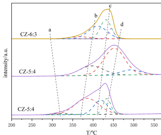
Figure 10. H 2 -TPR spectra of Cu-ZnO catalysts with different Cu:Zn ratio
