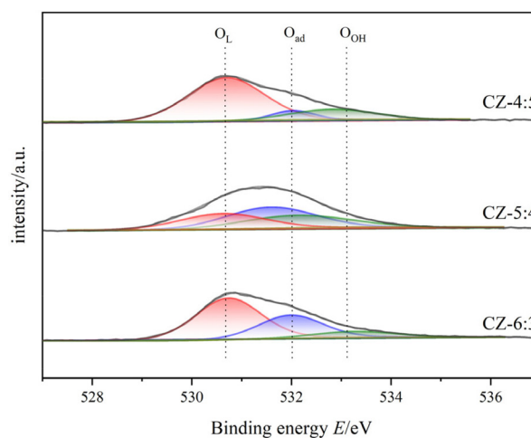
Figure 6. O 1s spectra of the catalysts with different Cu:Zn ratios
