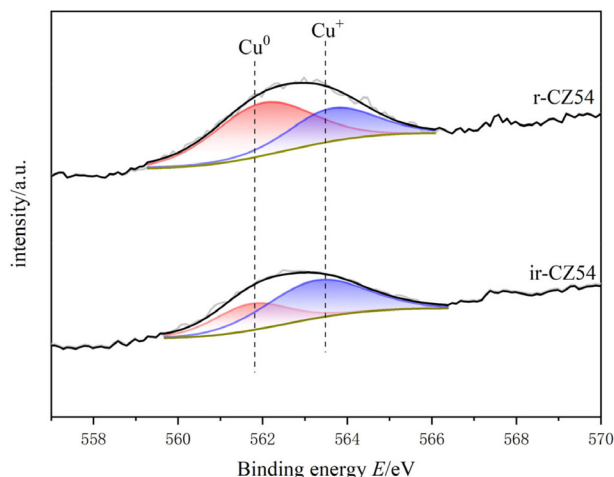
Figure 7. Cu LMM spectra of the CZ-5:4 catalysts after the reaction with reduction or not
