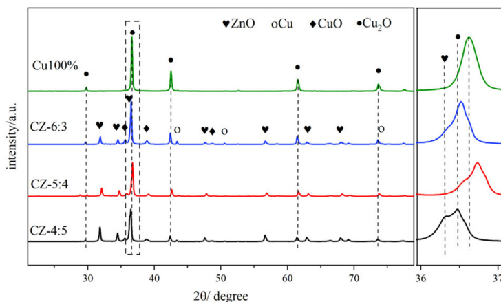
Figure 3. XRD patterns of Cu-ZnO catalysts with different Cu:Zn ratios and partial enlargement
