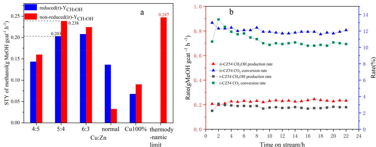
Figure 2. (a) STY_{\text{CH}_3\text{OH}} patterns of Cu-ZnO catalysts with different copper-zinc ratios and (b) during the 24 h stability test on CZ-5:4 catalyst
