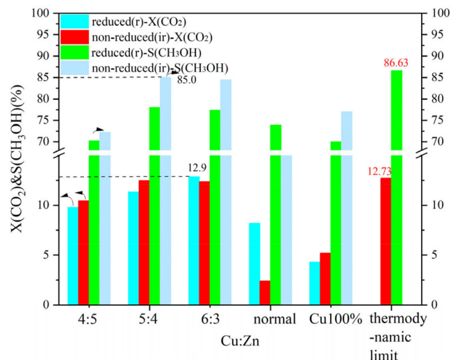
Figure 1. X_{\text{CO}_2} and S_{\text{CH}_3\text{OH}} patterns of Cu-ZnO catalysts with different copper-zinc ratios
