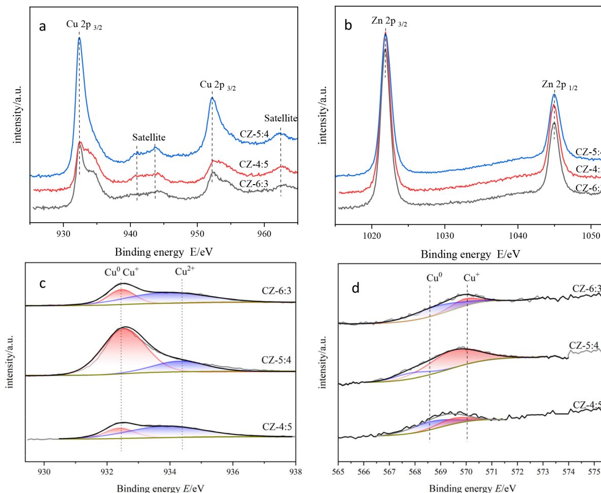
Figure 5. (a) the Cu 2p; (b) the Zn 2p; (c) Cu 2p 3/2 ; (d) the Cu auger electron spectra of the catalysts with different Cu:Zn ratios
