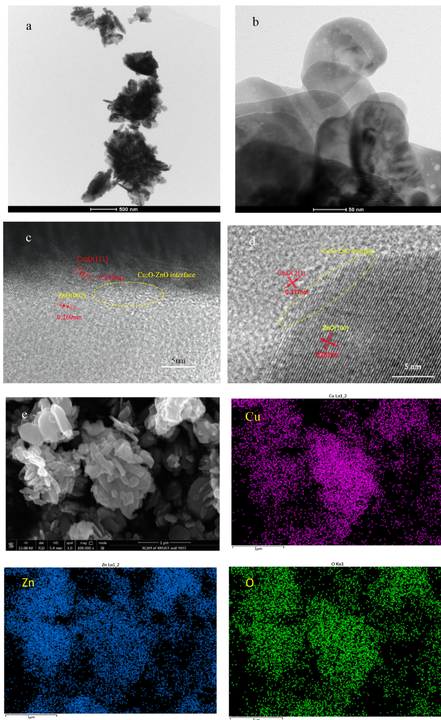
Figure 4. (a, b) TEM diagram; (c, d) HRTEM plot; (e) SEM diagram and its EDX element are mapped of CZ-5:4
