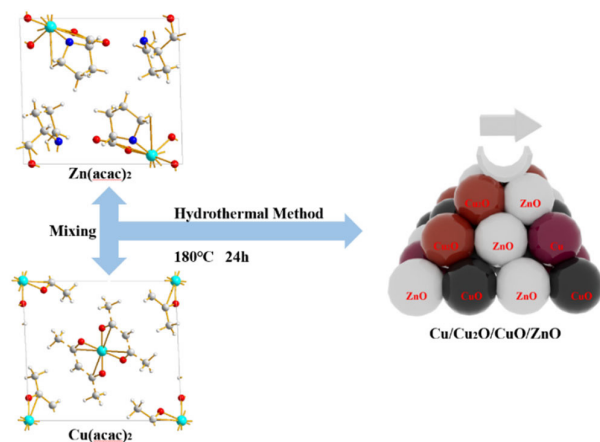
Scheme 1. Schematic diagram of the preparation of a Cu/Zn catalyst using the acetylacetonate salt precursor
