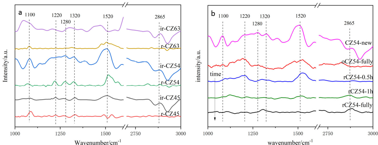
Figure 9. In-situ DRIFT spectra of the \text{CO}_2 adsorption on (a) Cu-ZnO catalysts with different Cu:Zn ratios; (b) a new, fully oxidized and reduced difference time the CZ-5:4 catalyst
