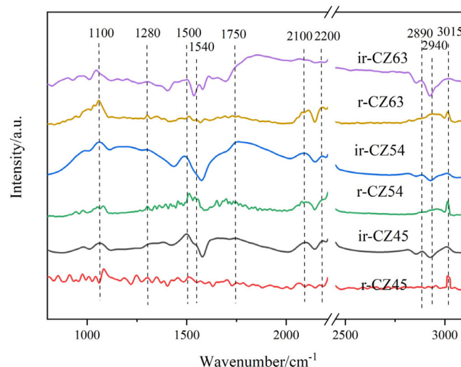
Figure 12. In situ DRIFT spectra of the CO 2 hydrogenation reaction on Cu-ZnO catalysts with different Cu:Zn ratios
