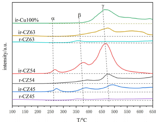
Figure 8. CO 2 -TPD patterns of the Cu-ZnO catalysts with different Cu:Zn ratios and pure copper cat
