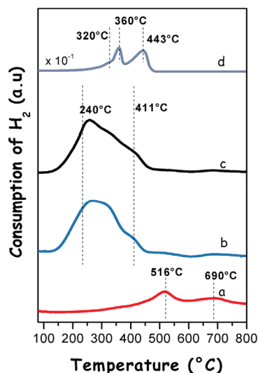
Figure 3. \text{H}_2 -TPR profiles of alumina-supported mixed samples prepared by different methods and with a 40% metallic charge, a: C-2, b: CM0.5-2, c: CM0.5-1, d: M-2
