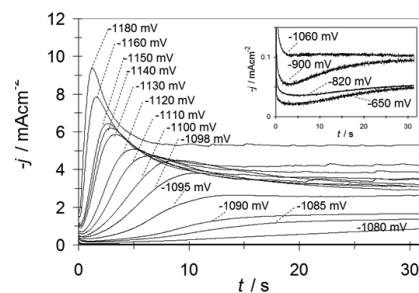
Figure 2. A set of transients obtained from HOPG/ 10^{-2} M of \text{CoSO}_4 + 1\text{M NH}_4\text{SO}_4 (pH 4.5) system by means of the potential step technique for different potential step values (mV) indicated in the figure. In all the cases, the initial potential was 0.600 V
