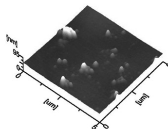
Figure 6. AFM image of the deposits obtained at -820 mV onto HOPG from an aqueous solution 10^{-2} M of \text{CoSO}_4 + 1M (\text{NH}_4)_2\text{SO}_4 (pH 4.5)
