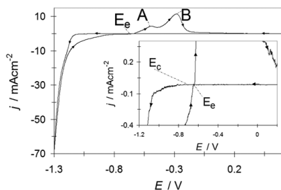
Figure 1. A typical cyclic voltammogram obtained from the HOPG/ 10^{-2} M of \text{CoSO}_4 + 1\text{M NH}_4\text{SO}_4 (pH 4.5) system. The potential scan rate was started at 0.600 V toward the negative direction with a potential scan rate of 20\text{ mV s}^{-1}
