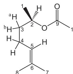
Figure 1. ( R )-6-methyl-5-hepten-2-yl (sulcatyl acetate), essential oil isolated from Aristolochia trilobata
