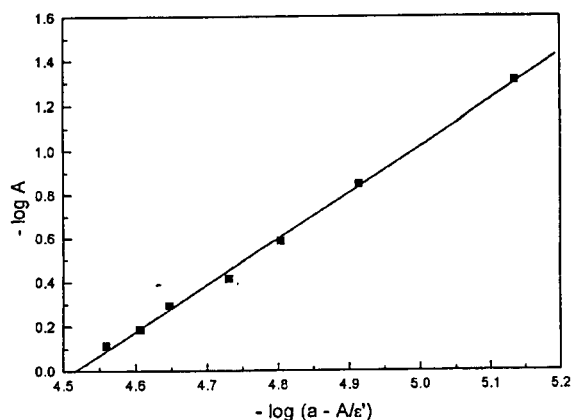
Figure 2. Correlation between the -\log A and the -\log (a - A / \epsilon') where a = [vanadium], A is the absorbance at 542 nm and \epsilon' is the molar absorptivity of the complex, assuming m = 1 . Concentration of H_2O_2 is 0.15% w/v; [H_2SO_4] = 0.5 \text{ mol L}^{-1} ; ionic strength = 0.01 \text{ mol L}^{-1} (KCl). Temperature = 28.0 \pm 0.5^\circ \text{C} .
