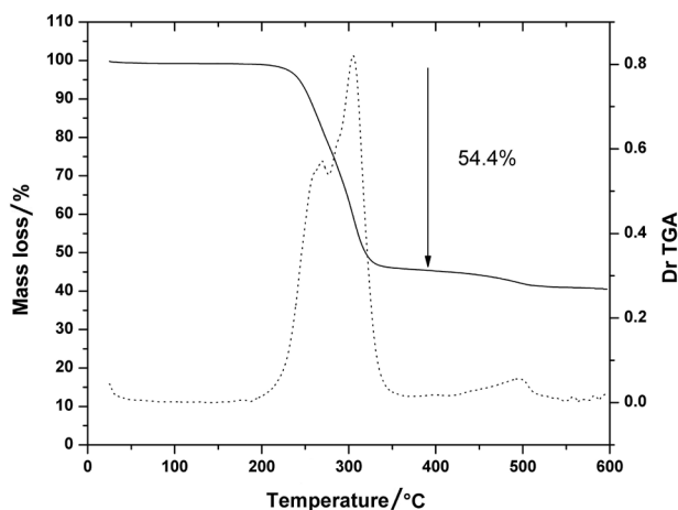
Figure 5. Thermogravimetric measurement was performed in the temperature range from 25 to 600 °C at heating rates of 10 °C min -1 for the compound [Cd 8 Cl 2 (μ 4 -Se)(SePh) 12 (PCy 3 ) 2 ] \cdot 2.5CH 3 OH.
