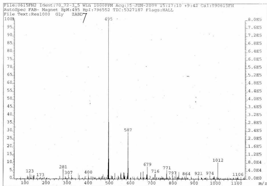
Figure S15. FABMS(-) spectrum of 2 (CD 3 OD).
