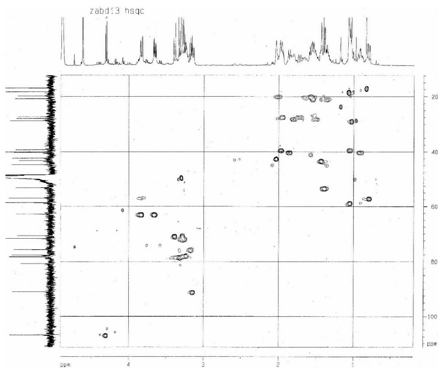
Figure S3. HSQC spectrum of 1 ( \text{CD}_3\text{OD} ).
