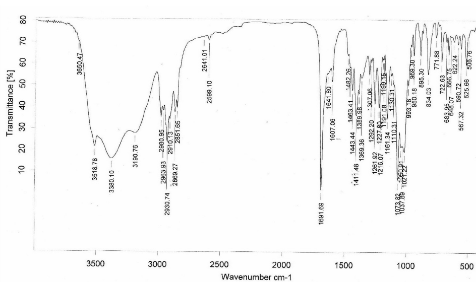
Figure S16. IR spectrum of 2 (KBr pellet).
