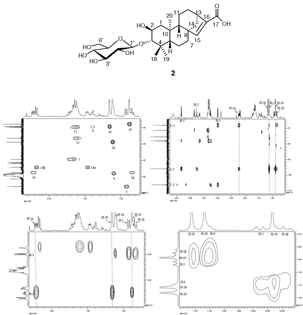
Figure S17. Key expansion 2D NMR spectra of 2 (CD 3 OD).
