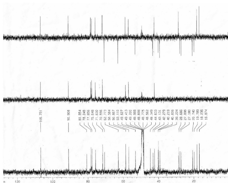
Figure S2. ^{13}\text{C} NMR spectrum of 1 (100MHz, \text{CD}_3\text{OD} ).
