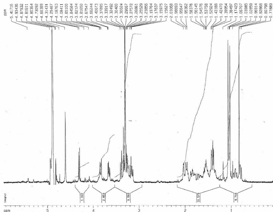
Figure S1. 1 H NMR spectrum of 1 (400MHz, CD 3 OD).
