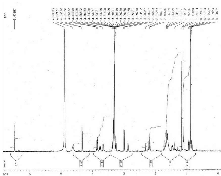
Figure S9. 1 H NMR spectrum of 2 (500MHz, CD 3 OD).
