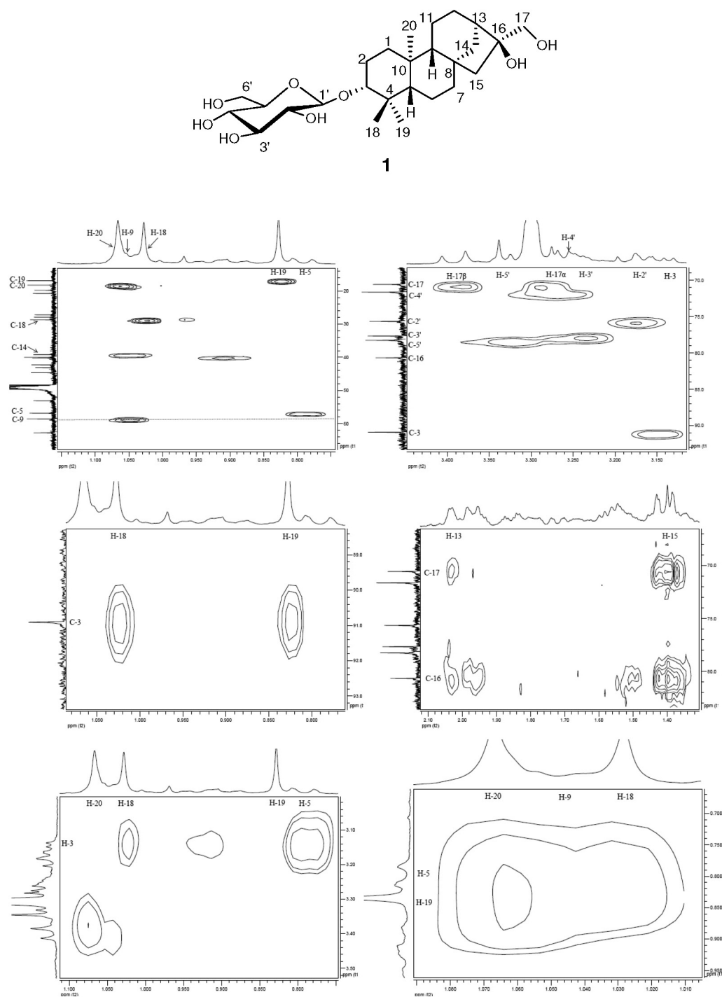
Figure S8. Key expansion 2D NMR spectra of 1 (CD 3 OD).
