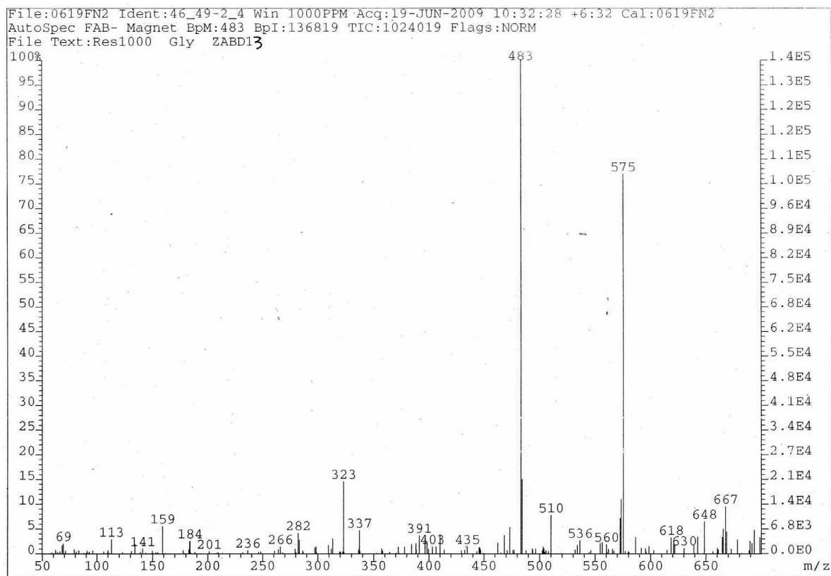
Figure S7. FABMS(-) spectrum of 1 (CD 3 OD).
