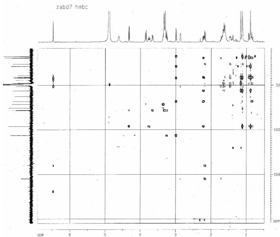
Figure S13. HMBC spectrum of 2 (CD 3 OD).
