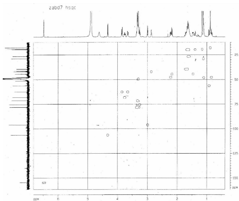
Figure S11. HSQC spectrum of 2 (CD 3 OD).
