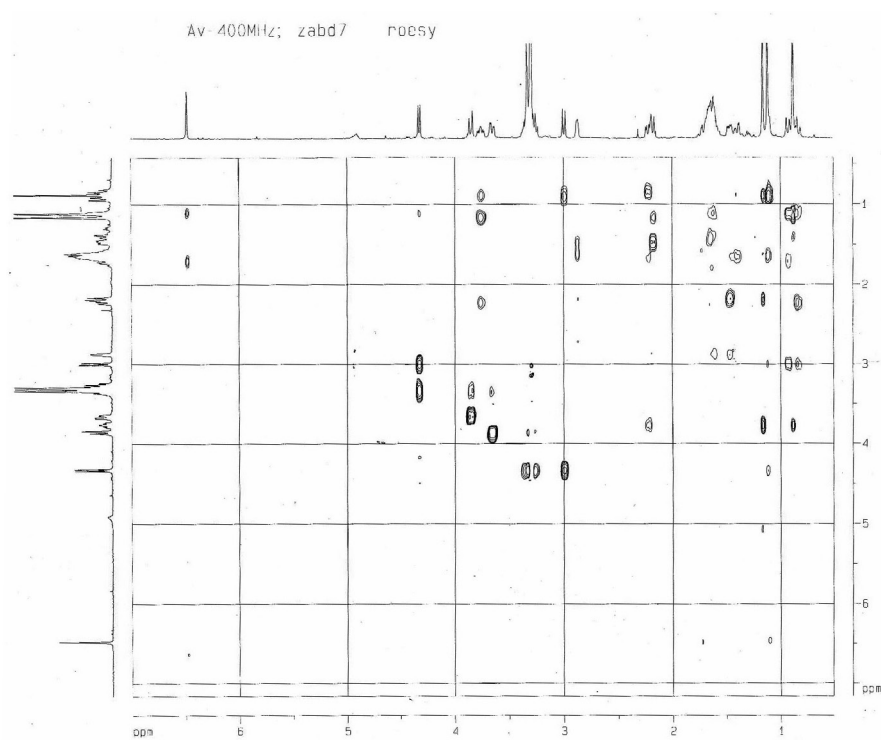
Figure S14. ROSEY spectrum of 2 (CD 3 OD).
