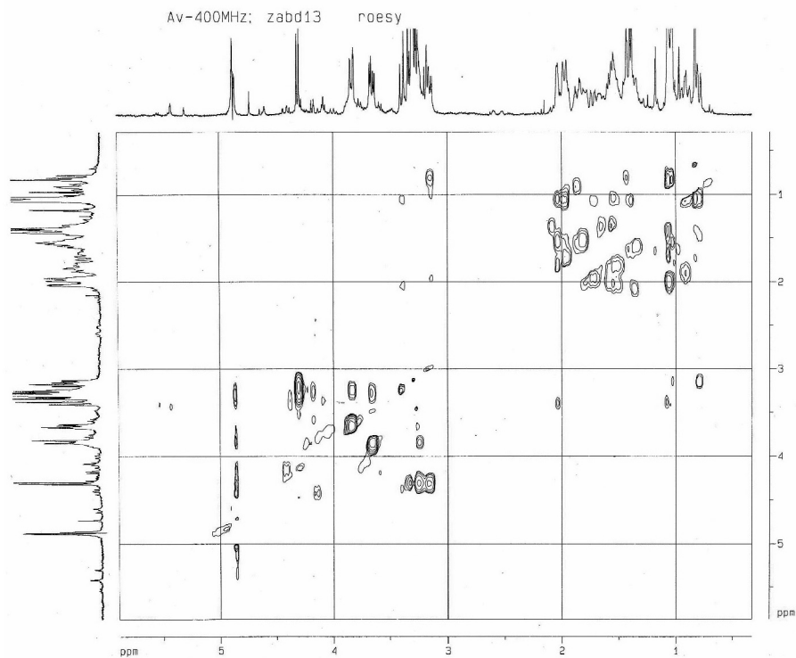
Figure S6. ROESY spectrum of 1 (CD 3 OD).
