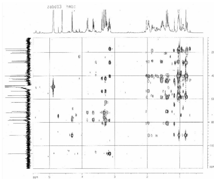
Figure S4. HMBC spectrum of 1 (CD 3 OD).
