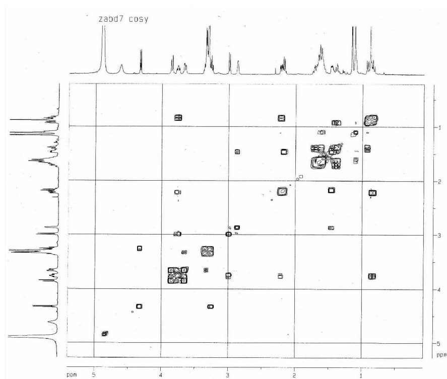
Figure S12. 1 H, 1 H COSY spectrum of 2 (CD 3 OD).
