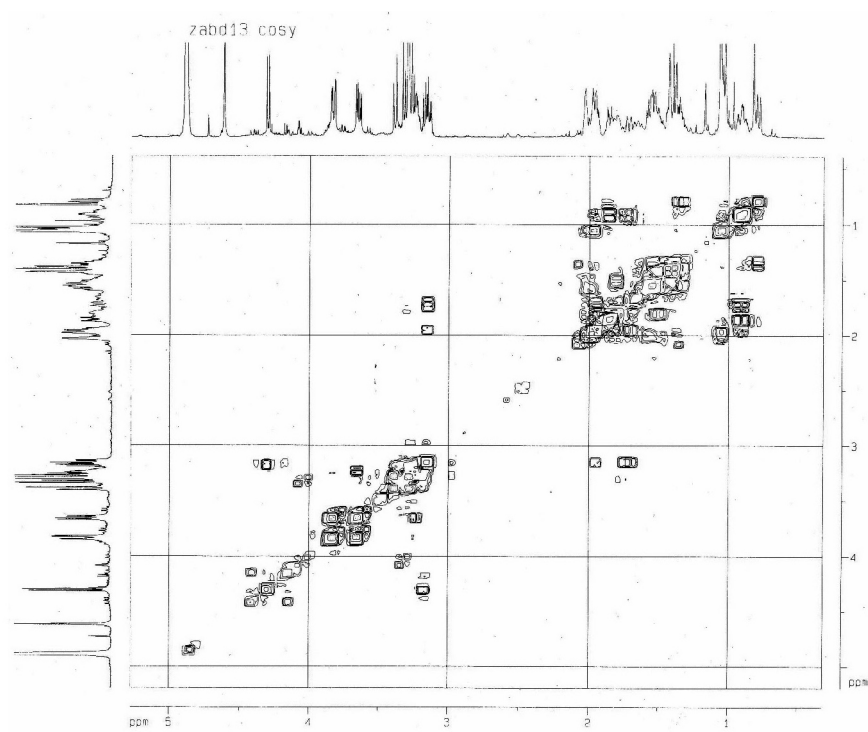
Figure S5. 1 H, 1 H COSY spectrum of 1 (CD 3 OD).
