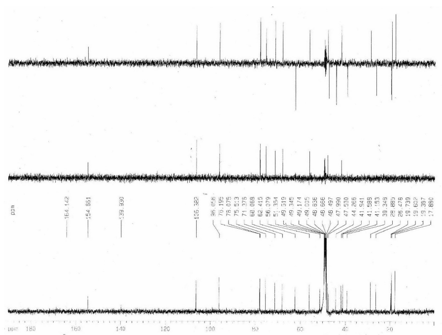
Figure S10. 13 C NMR (DEPT) spectrum of 2 (125MHz, CD 3 OD).
